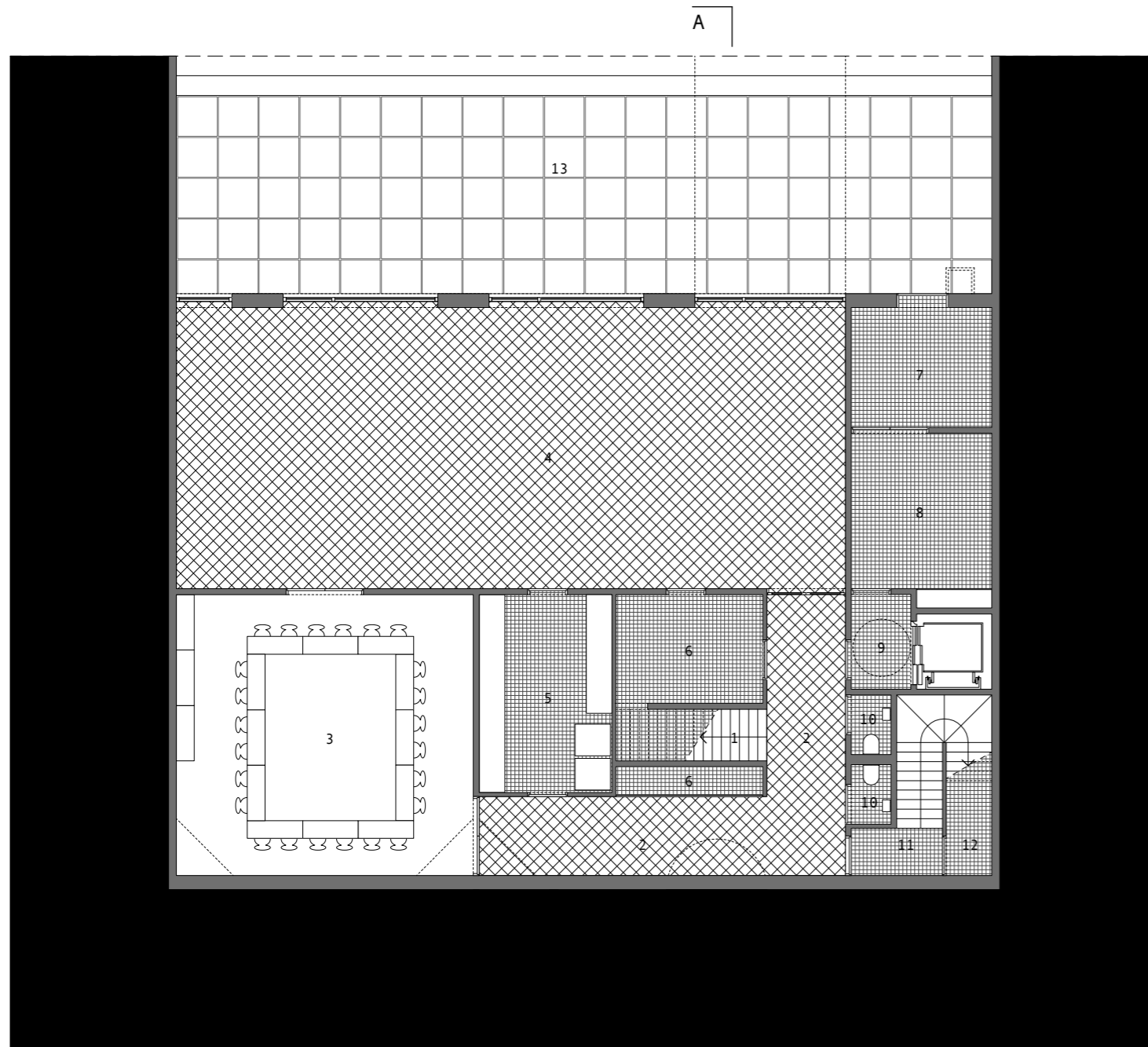
PLAN SOUTERRAIN
